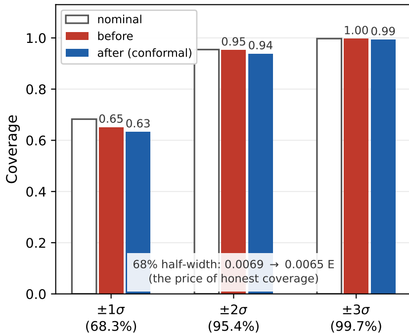
Coverage at the Gaussian levels
