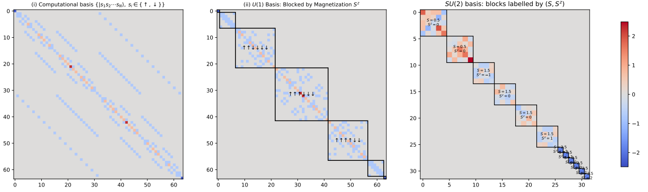
Figure 1: Three different presentations of the XXZ Hamiltonian. (i): In the default computational basis of spin vectors. (ii) In a reordering of the computational basis into equal spin up (down) classes, i.e. no spin up, one spin up etc..., here U is simply a permutation matrix. (iii) After changing the basis into the (S^2, S_Z) basis.
