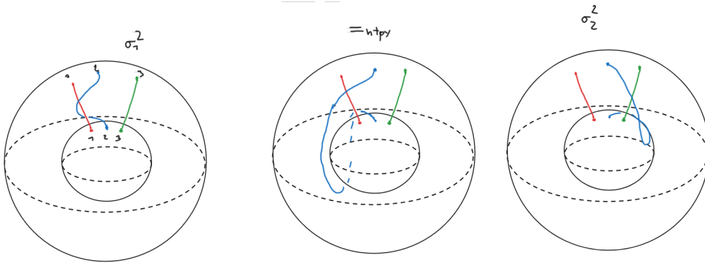
Figure 2: 3 Anyons on the sphere S^2 with the equivalence of the braids \sigma_1^2 and \sigma_2^2 . From an exercise github in [Sim23].
