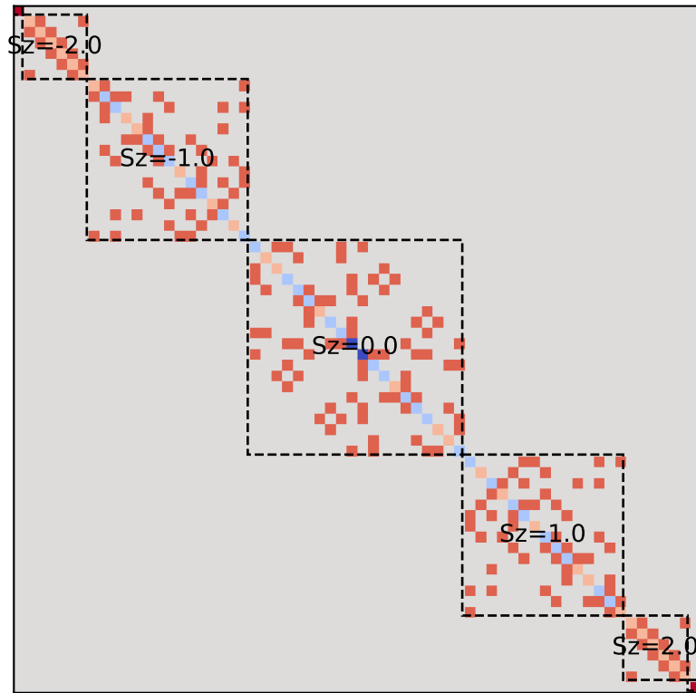
(ii) Basis ordered by total magnetization S_{\text{tot}}^z
