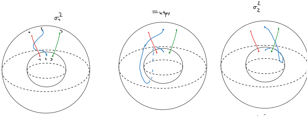
Figure 4.1: 3 Anyons on the sphere S^2 with the equivalence of the braids \sigma_1^2 and \sigma_2^2 . From an exercise github in [Sim23].
