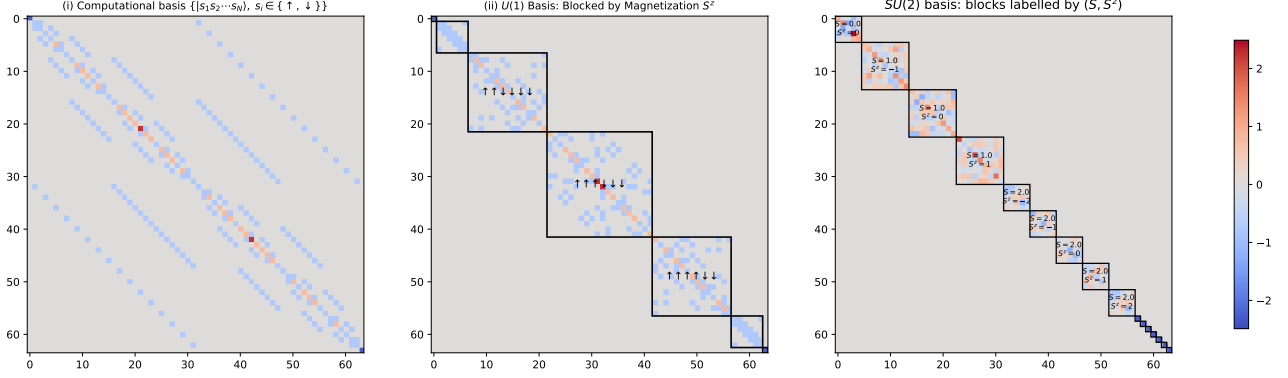
Figure 3.1: Three different presentations of the XXZ Hamiltonian for N = 6 . (i): In the default computational basis of spin vectors. (ii) In a reordering of the computational basis into equal spin up (down) classes, i.e. no spin up, one spin up etc..., here U is simply a permutation matrix. (iii) After changing the basis into the (S^2, S_z) basis.
