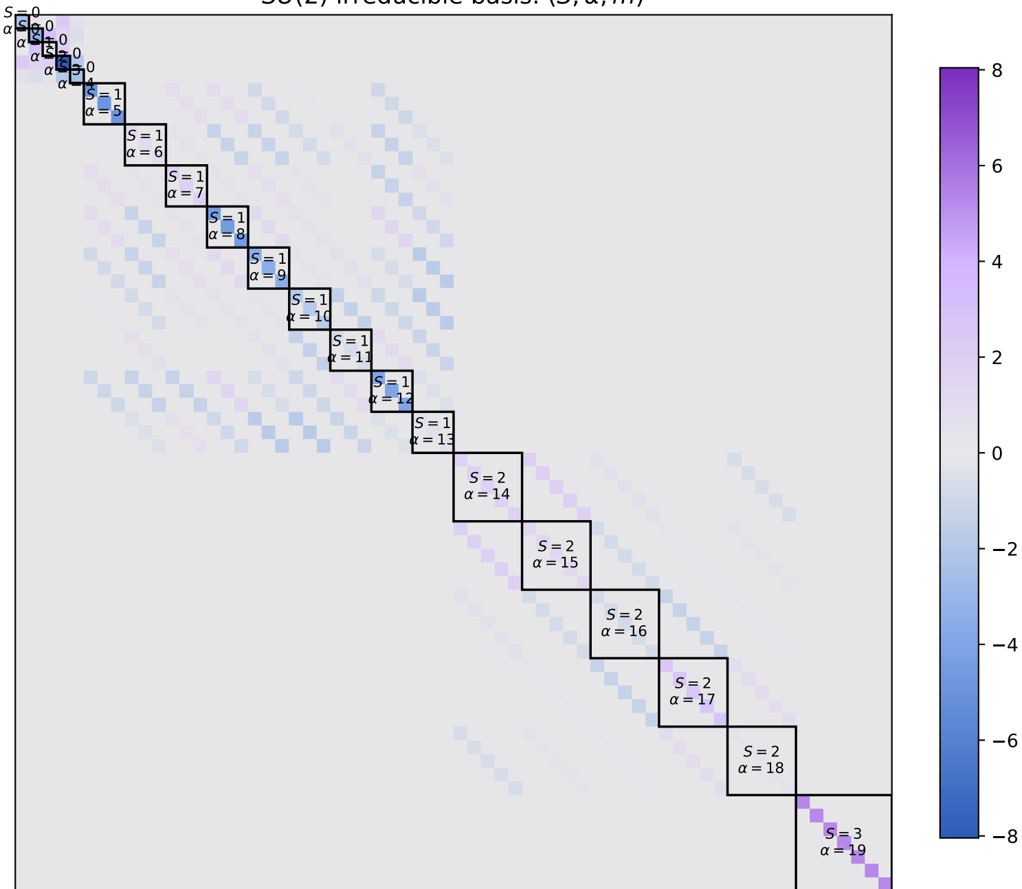
SU(2) irreducible basis: (S, \alpha, m)
