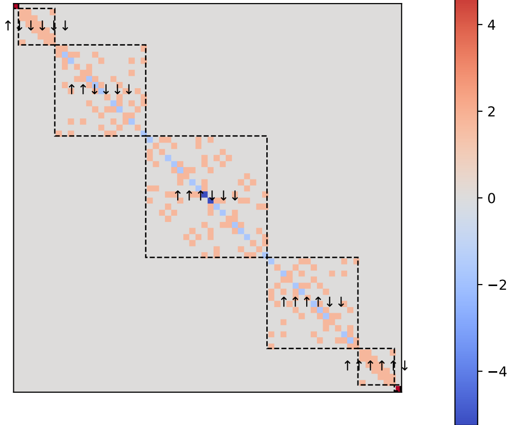
(ii) Basis ordered by total magnetization S_{\text{tot}}^z
