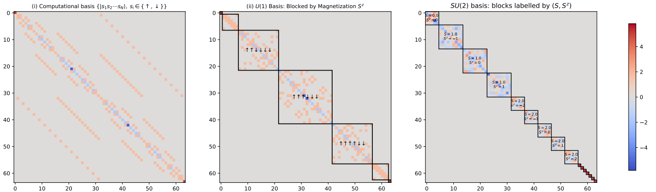
Figure 1: Three different presentations of the XXZ Hamiltonian. (i): In the default computational basis of spin vectors. (ii) In a reordering of the computational basis into equal spin up (down) classes, i.e. no spin up, one spin up etc..., here U is simply a permutation matrix. (iii) After changing the basis into the S^2 basis.
