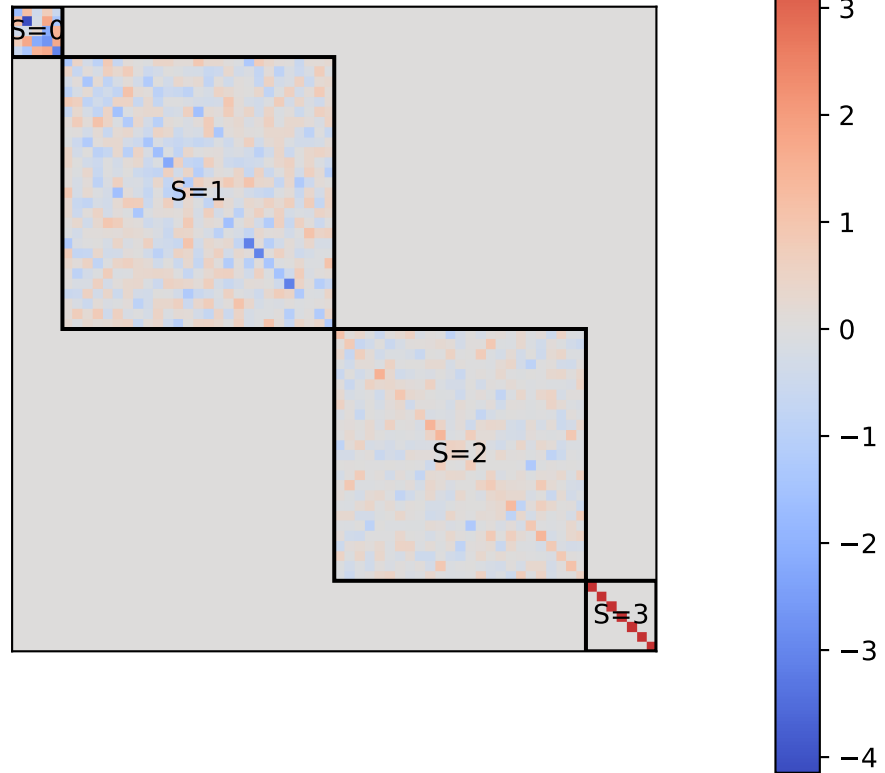
(iii) SU(2) Basis: Total Spin S^2
