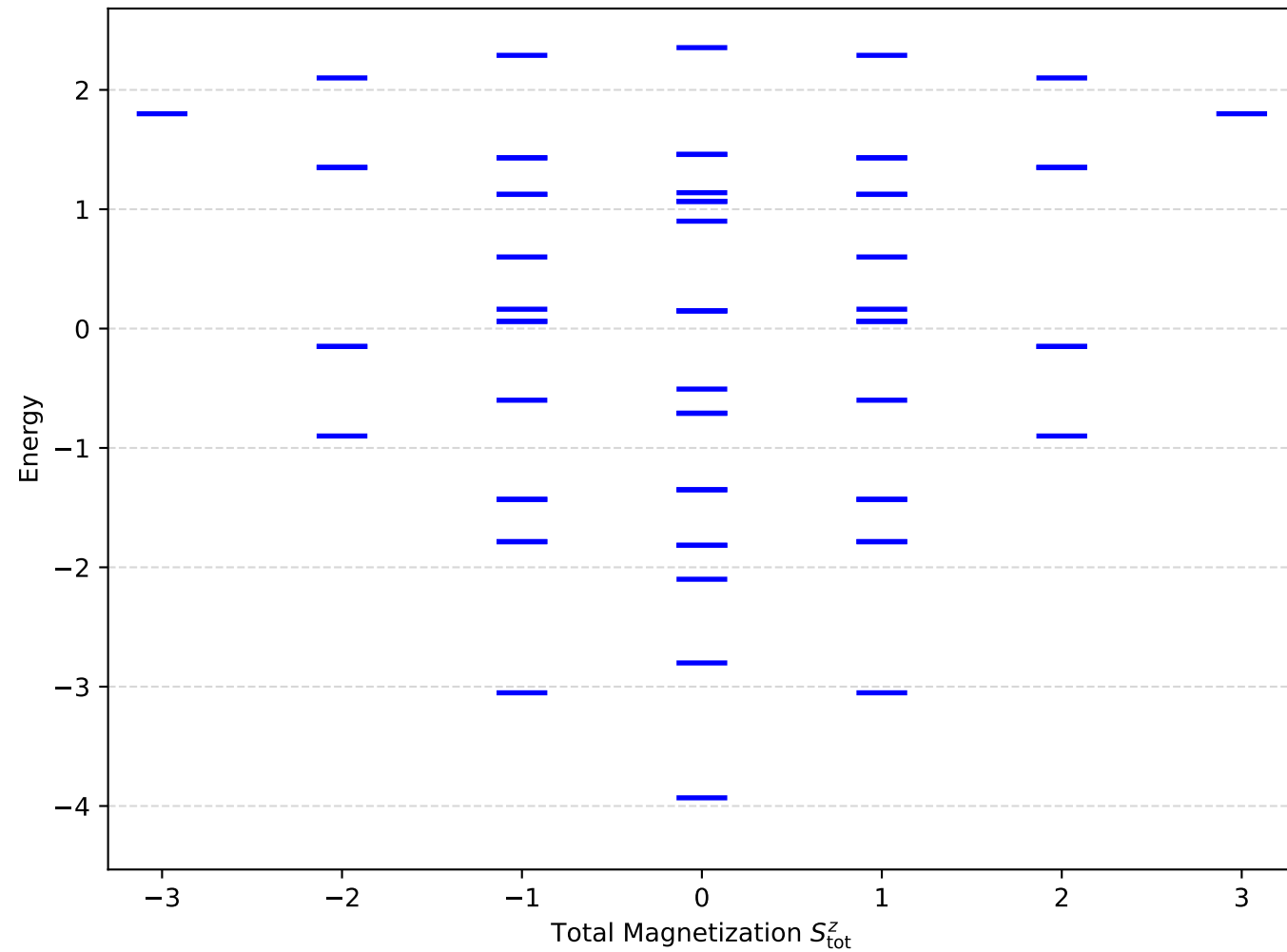
XXZ Model ( \Delta = 0.8 ): U(1) Symmetry Levels are split by anisotropy
