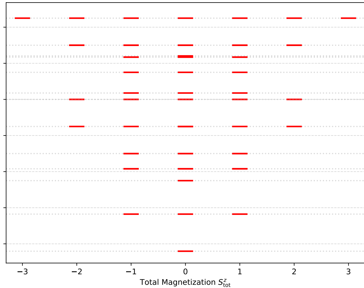
XXX Model ( \Delta = 1.0 ): SU(2) Symmetry Notice the exact horizontal ( 2S + 1 ) multiplets
