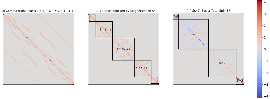
Figure 1.1: Three different presentations of the XXZ Hamiltonian. (i): In the default computational basis of spin vectors. (ii) In a reordering of the computational basis into equal spin up (down) classes, i.e. no spin up, one spin up etc... (iii) After changing the basis into the S^2 basis.
