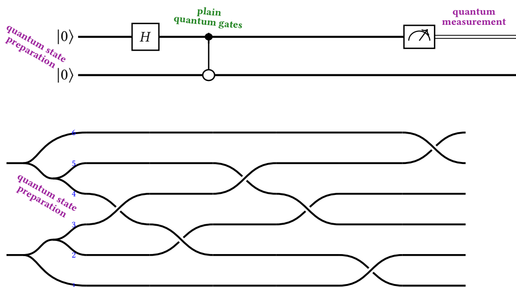
Figure 6.2: A standard 2-qubit quantum circuit and its lowering to a braid-circuit with inection weaves (missing yet).
