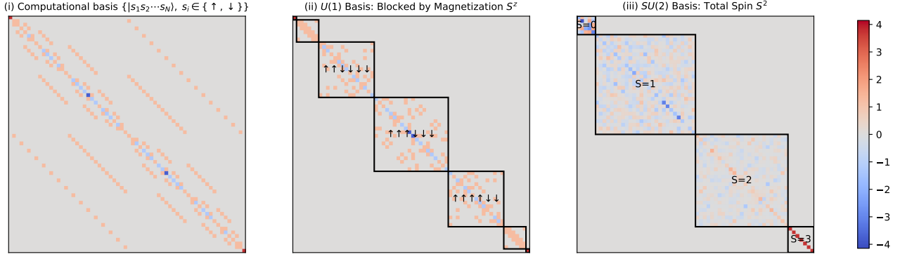
Figure 1.1: Three different presentations of the XXZ Hamiltonian. (i): In the default computational basis of spin vectors. (ii) In a reordering of the computational basis into equal spin up (down) classes, i.e. no spin up, one spin up etc..., here U is simply a permutation matrix. (iii) After changing the basis into the S^2 basis.
