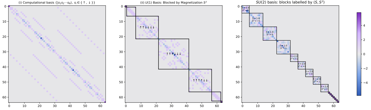
Figure 2.1: Three different presentations of the XXZ Hamiltonian. (i): In the default computational basis of spin vectors. (ii) In a reordering of the computational basis into equal spin up (down) classes, i.e. no spin up, one spin up etc..., here U is simply a permutation matrix. (iii) After changing the basis into the S^2 basis.
