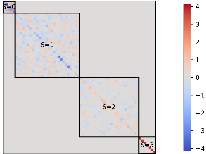
(iii) SU(2) Basis: Total Spin S^2
