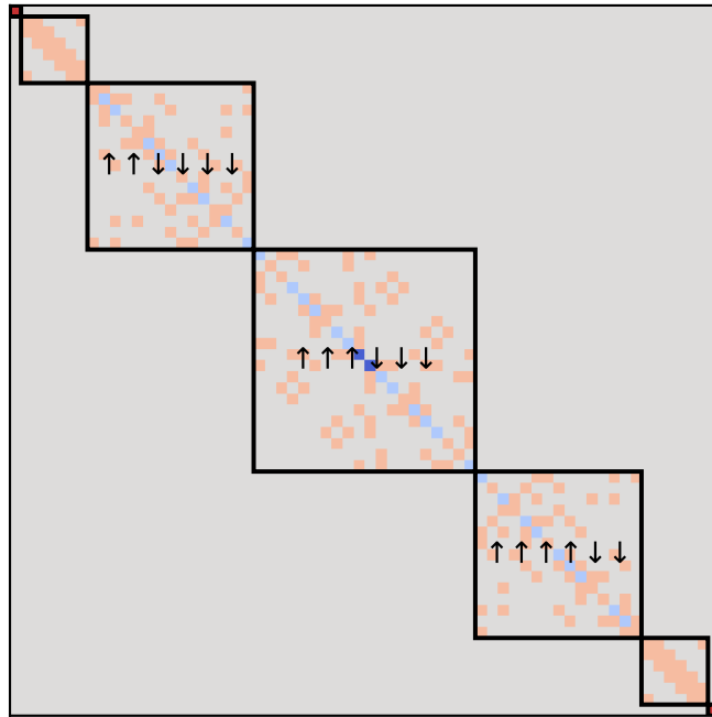
(ii) U(1) Basis: Blocked by Magnetization S^z
