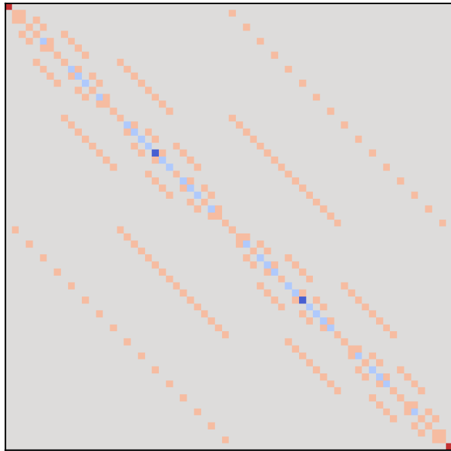
(i) Computational basis \{|s_1 s_2 \cdots s_N\rangle, s_i \in \{\uparrow, \downarrow\}\}
