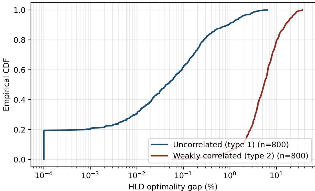
Pisinger 1995 — HLD optimality gap by correlation class
