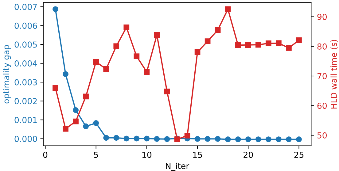
mckp_N10000_M10_weakly_f0.500_seed42
