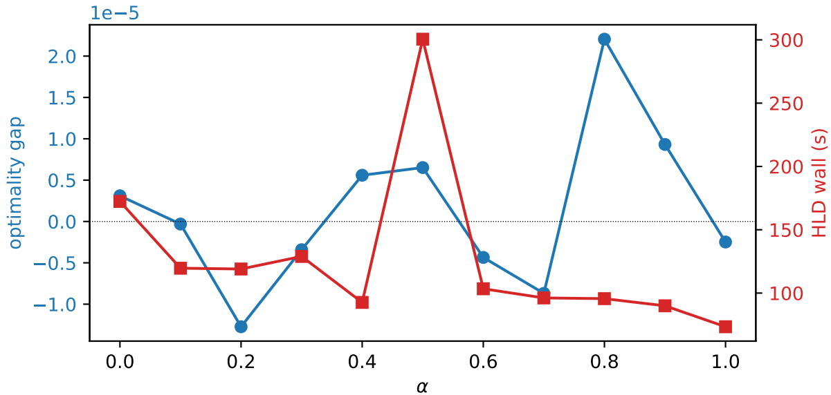
mckp_N10000_M10_weakly_f0.500_seed0
