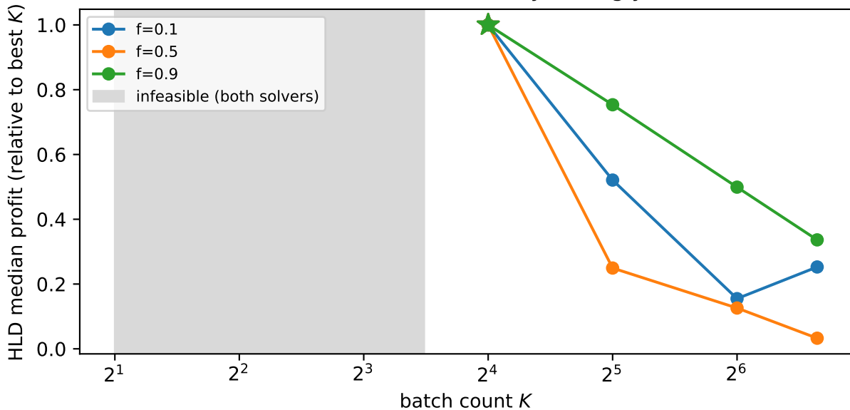
HLD solution quality vs batch count K ( N = 100,000 , inversely-strongly)
