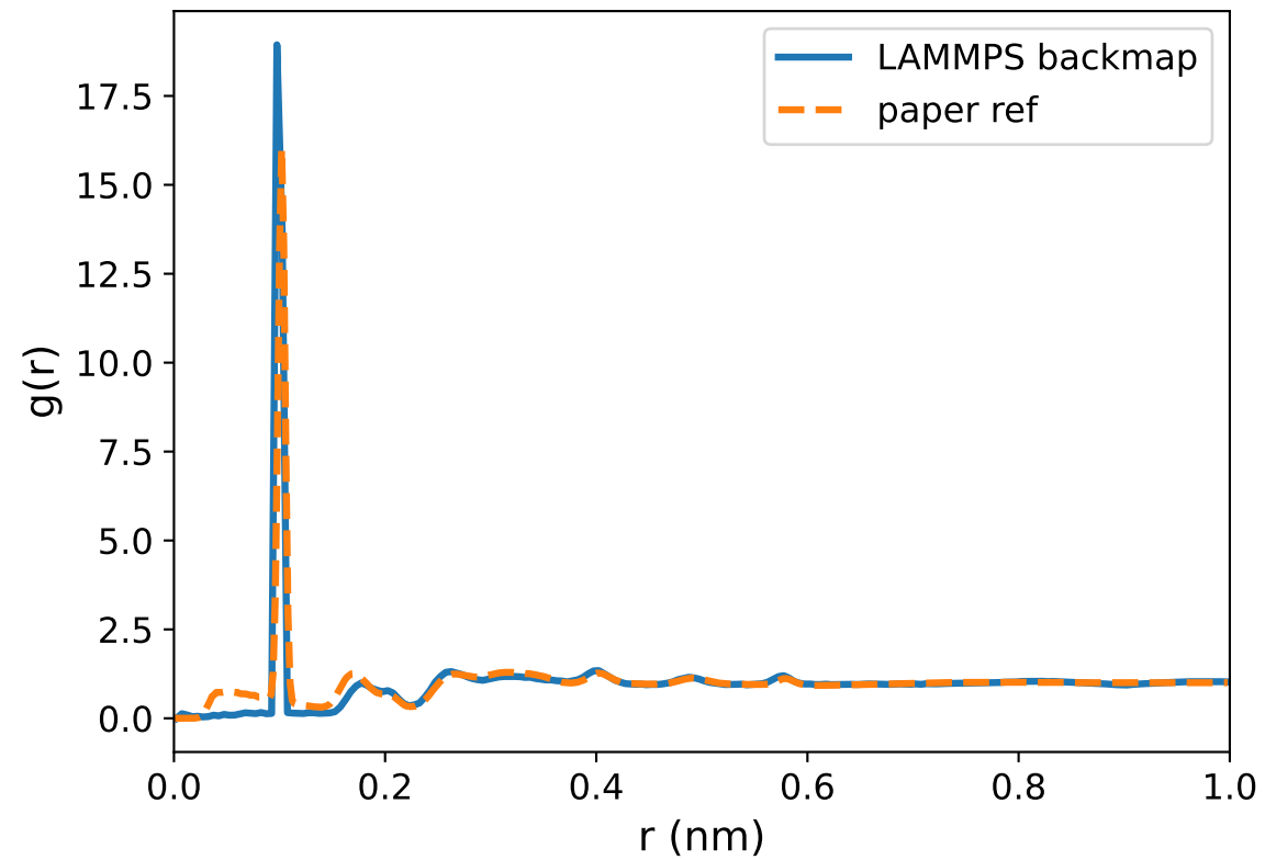
O-H
