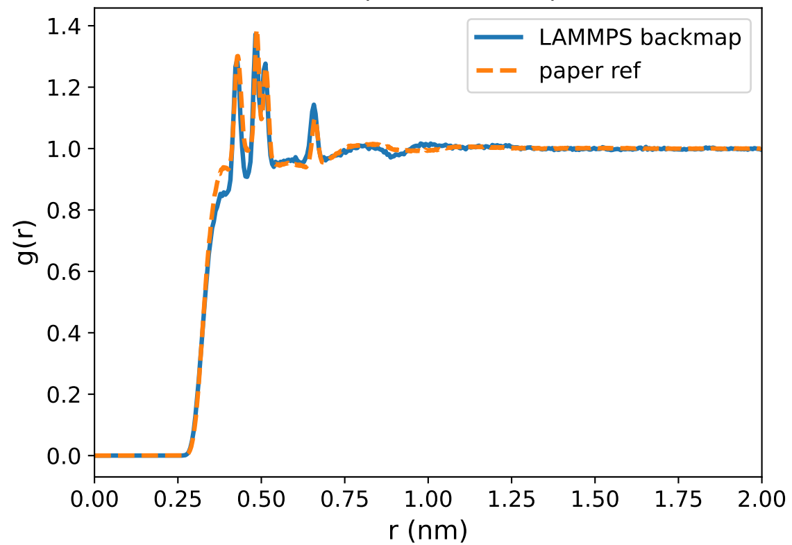
ring-ring (COM)
