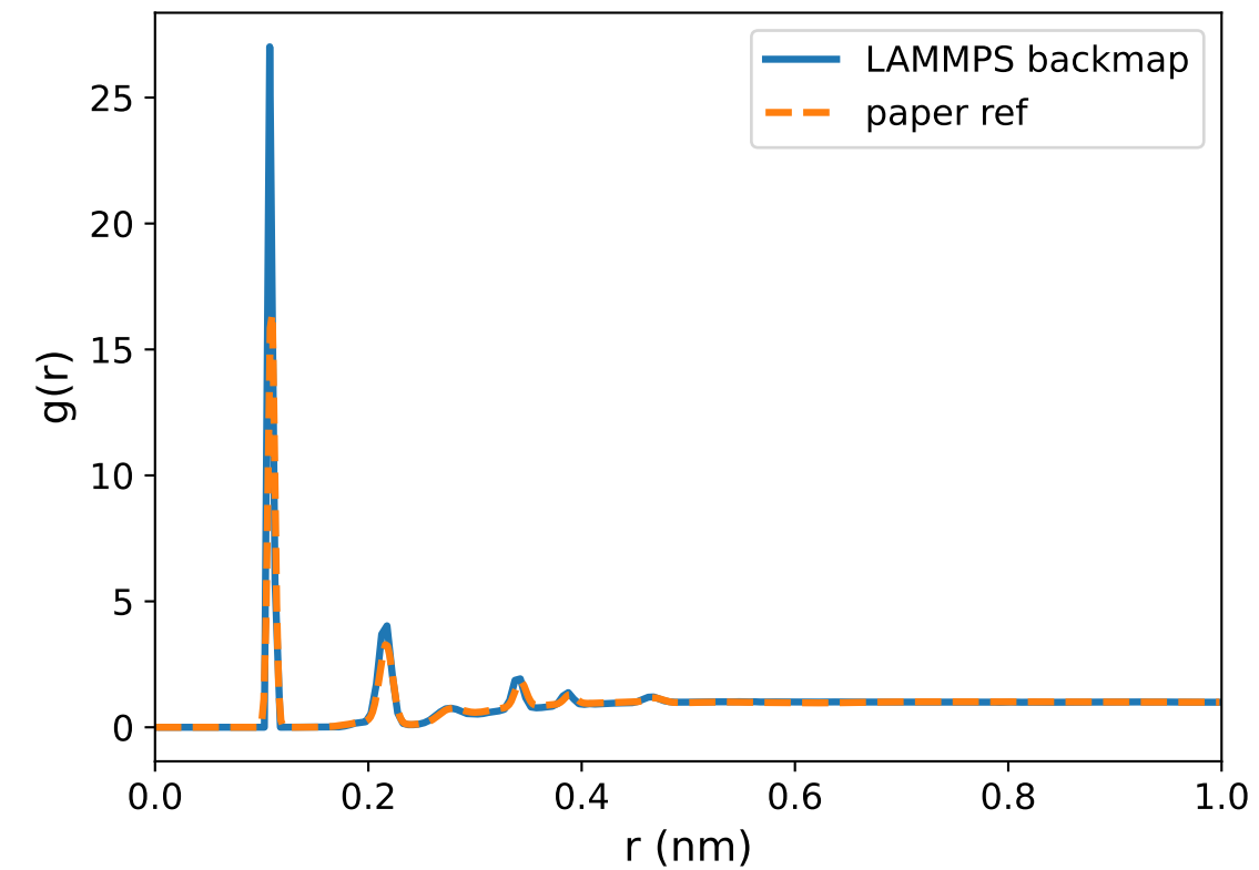
C-H
