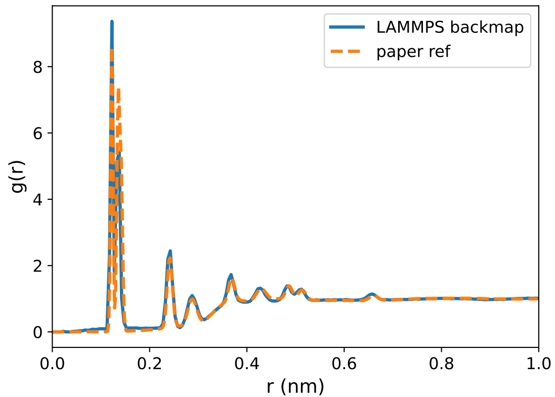
O-H
