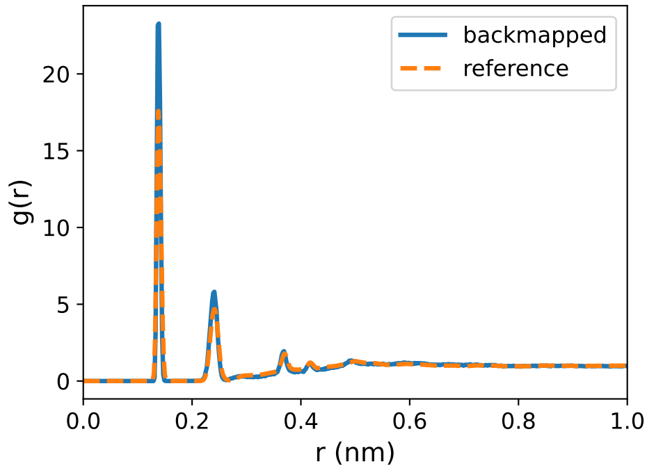
C-O vs AA
