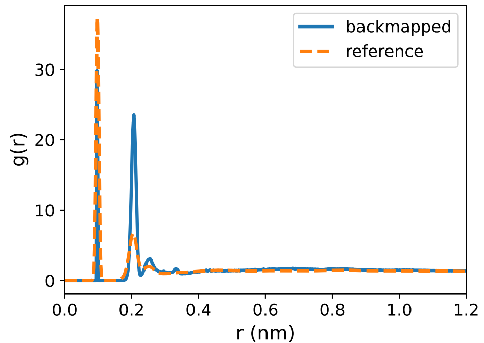
O-H
