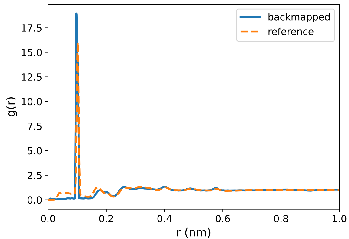
O-H
