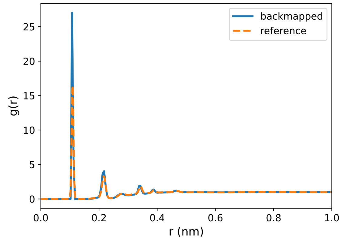
C-H
