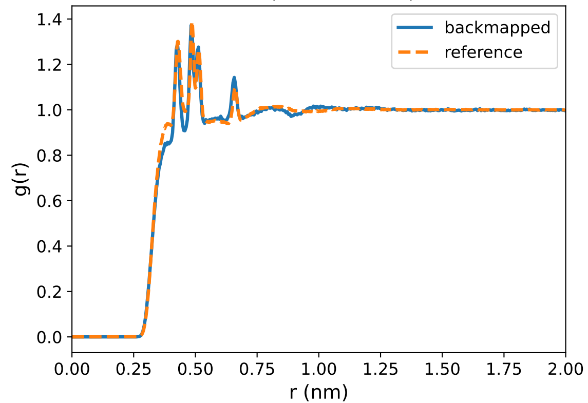
ring-ring (COM)
