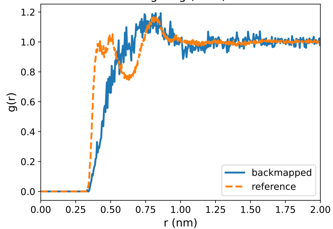
ring-ring (COM)
