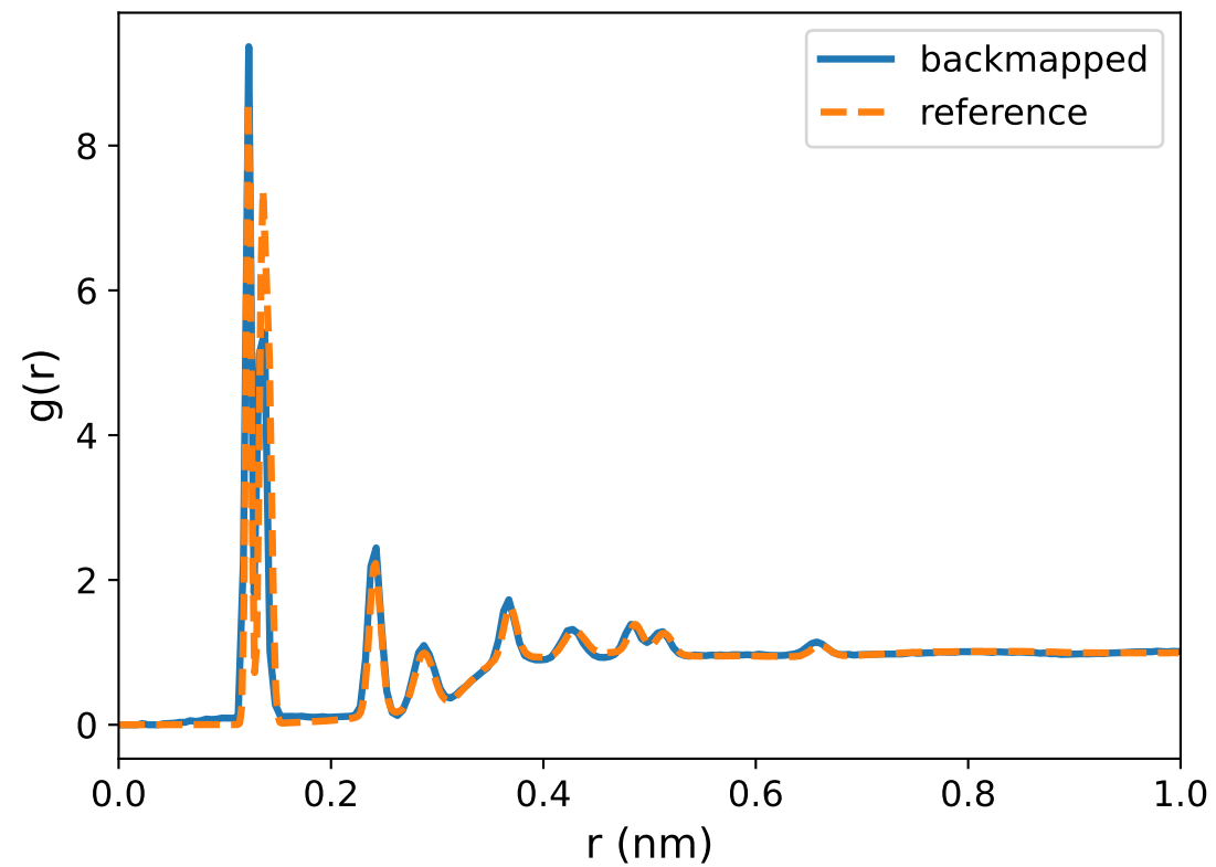
O-H
