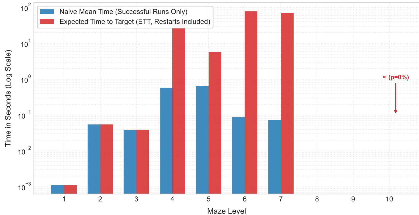
Naive Synthesis Time vs. Expected Time to Target (ETT) Across Levels 1–10
