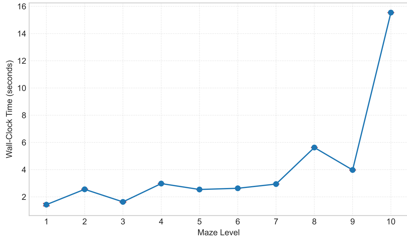
(A) Successful Single-Run Time (sec)
