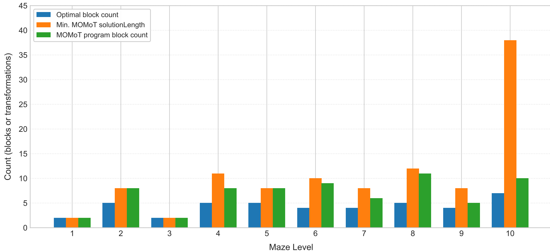
Optimal vs. MOMoT Search Length vs. MOMoT Program Size per Level
