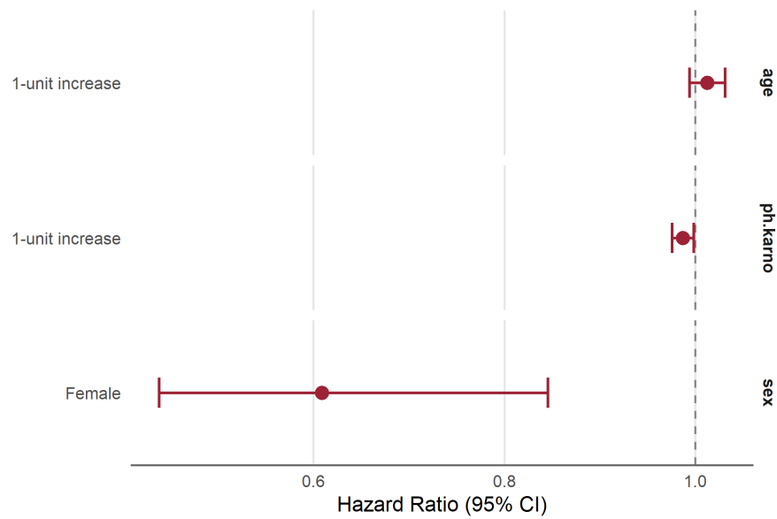
Figure 4: Forest plot of the multivariable Cox model (adjusted hazard ratios with 95% confidence intervals).
