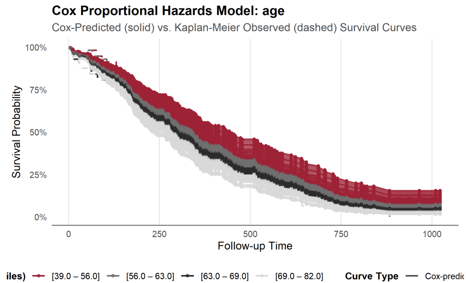
Figure 2: Model-predicted survival curve for the univariable age model, overlaid with the non-parametric Kaplan-Meier estimate.
