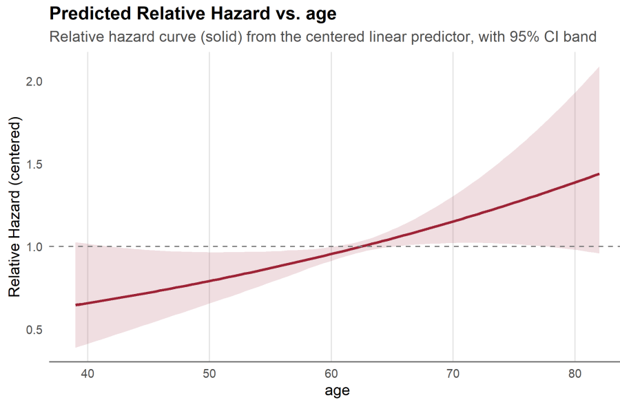
Figure 3: Marginal hazard ratio for age across its observed range, relative to the reference value.
