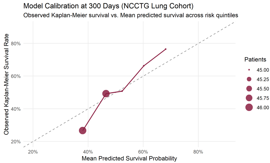
Figure 5: Calibration at 300 days: mean predicted survival versus observed Kaplan-Meier survival within predicted-survival quintiles; the dashed line marks perfect calibration.
