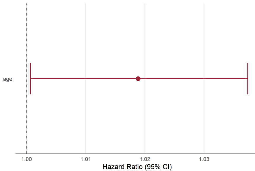
Figure 1: Forest plot of the univariable Cox model for age (hazard ratio with 95% confidence interval).
