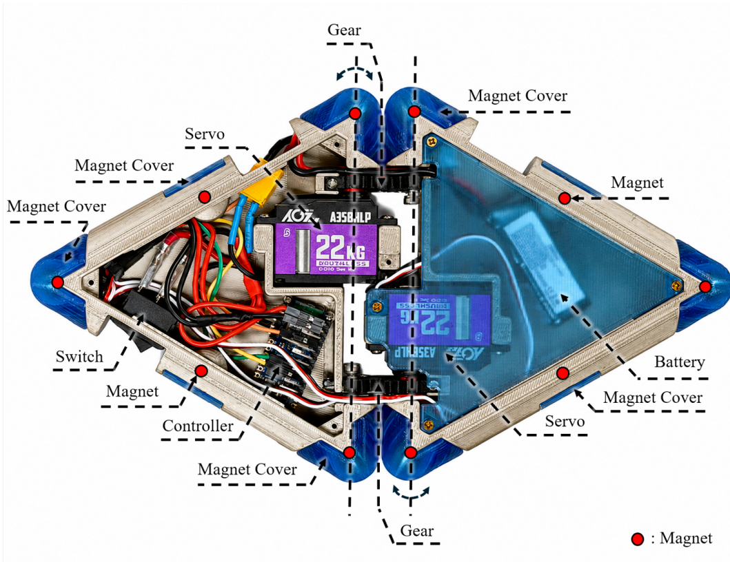
Fig. 1: Internal structural layout and component allocation of an individual module, highlighting the dual-servo drive mechanism, onboard electronics, and magnetic docking interfaces (red dots).
