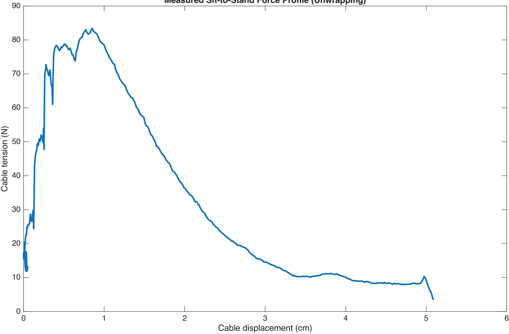
Measured Sit-to-Stand Force Profile (Unwrapping)
