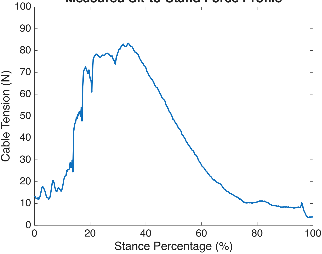
Measured Sit-to-Stand Force Profile
