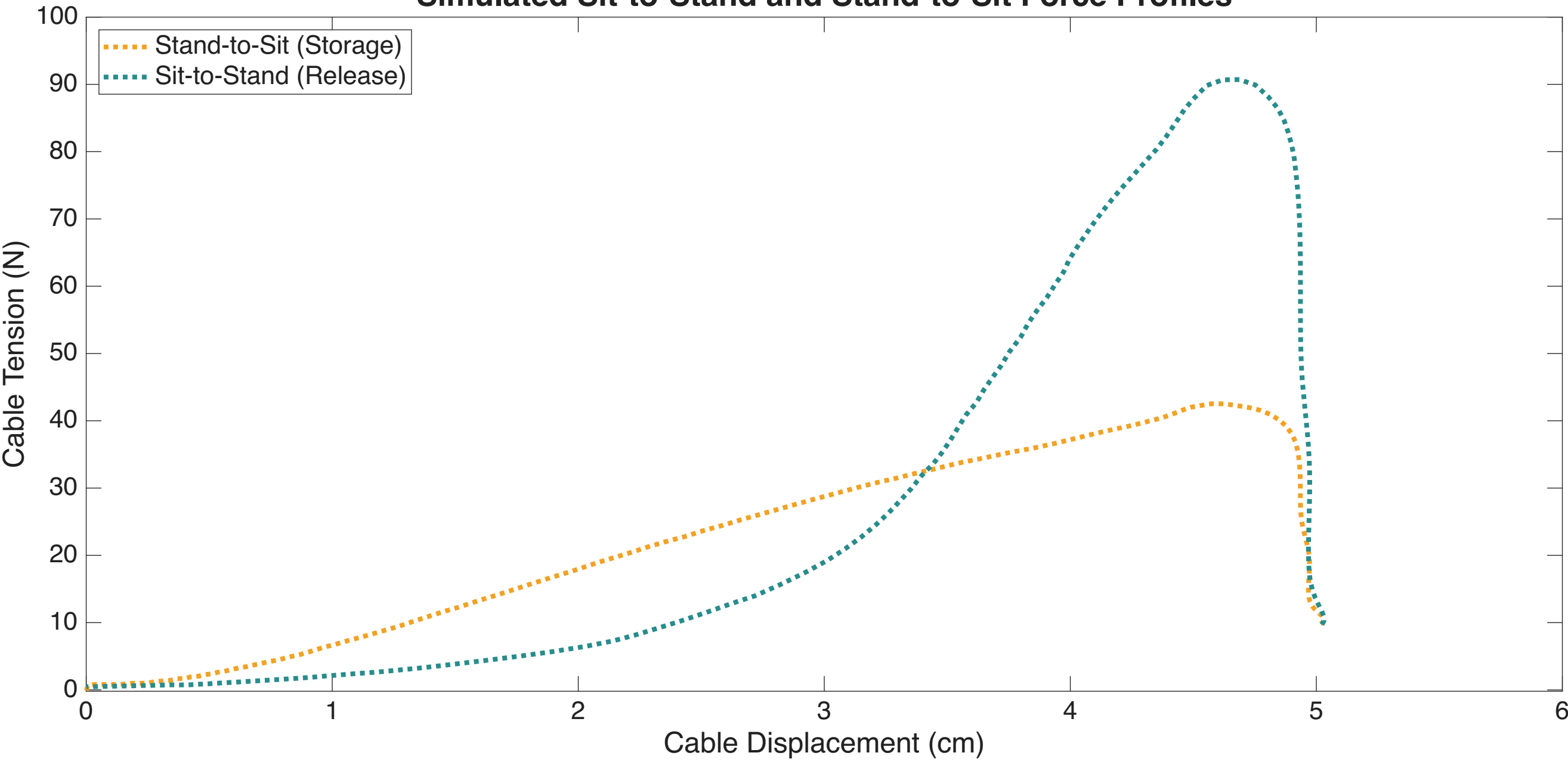
Simulated Sit-to-Stand and Stand-to-Sit Force Profiles
