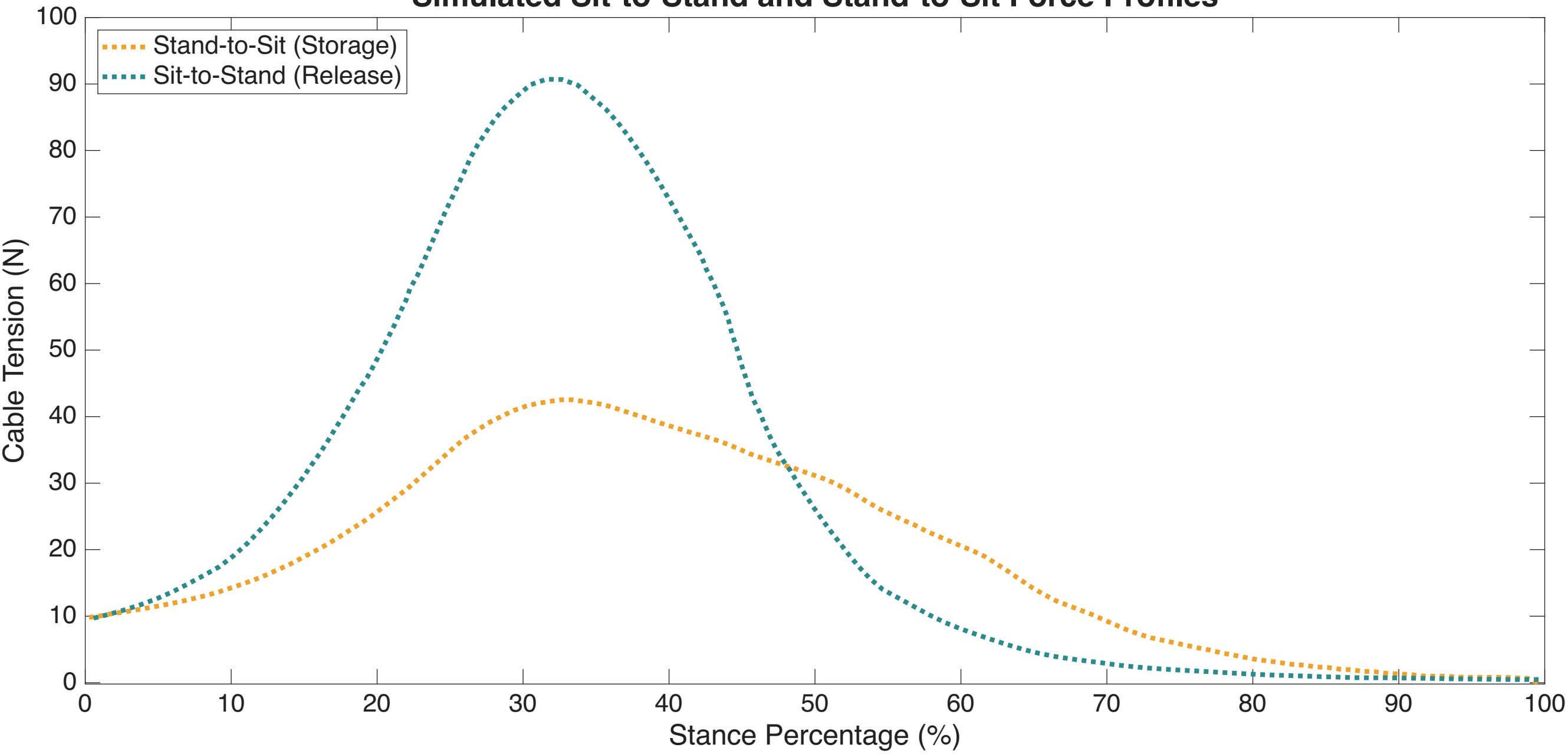
Simulated Sit-to-Stand and Stand-to-Sit Force Profiles
