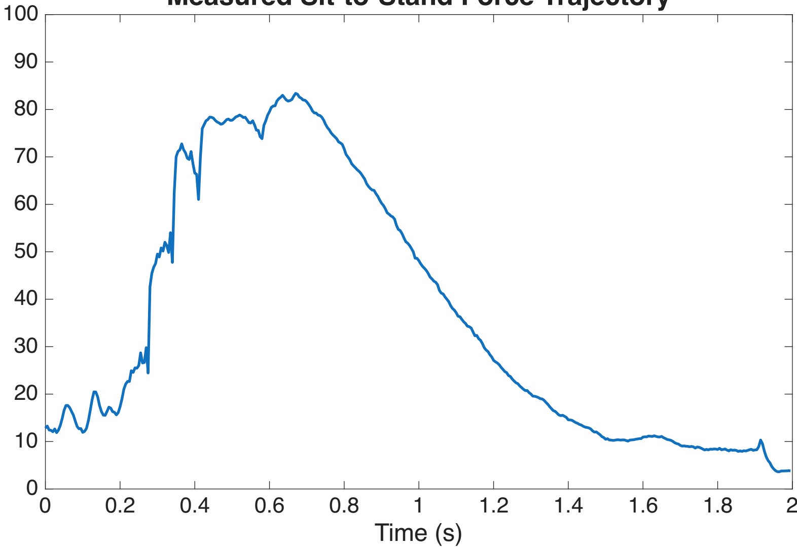
Measured Sit-to-Stand Force Trajectory
