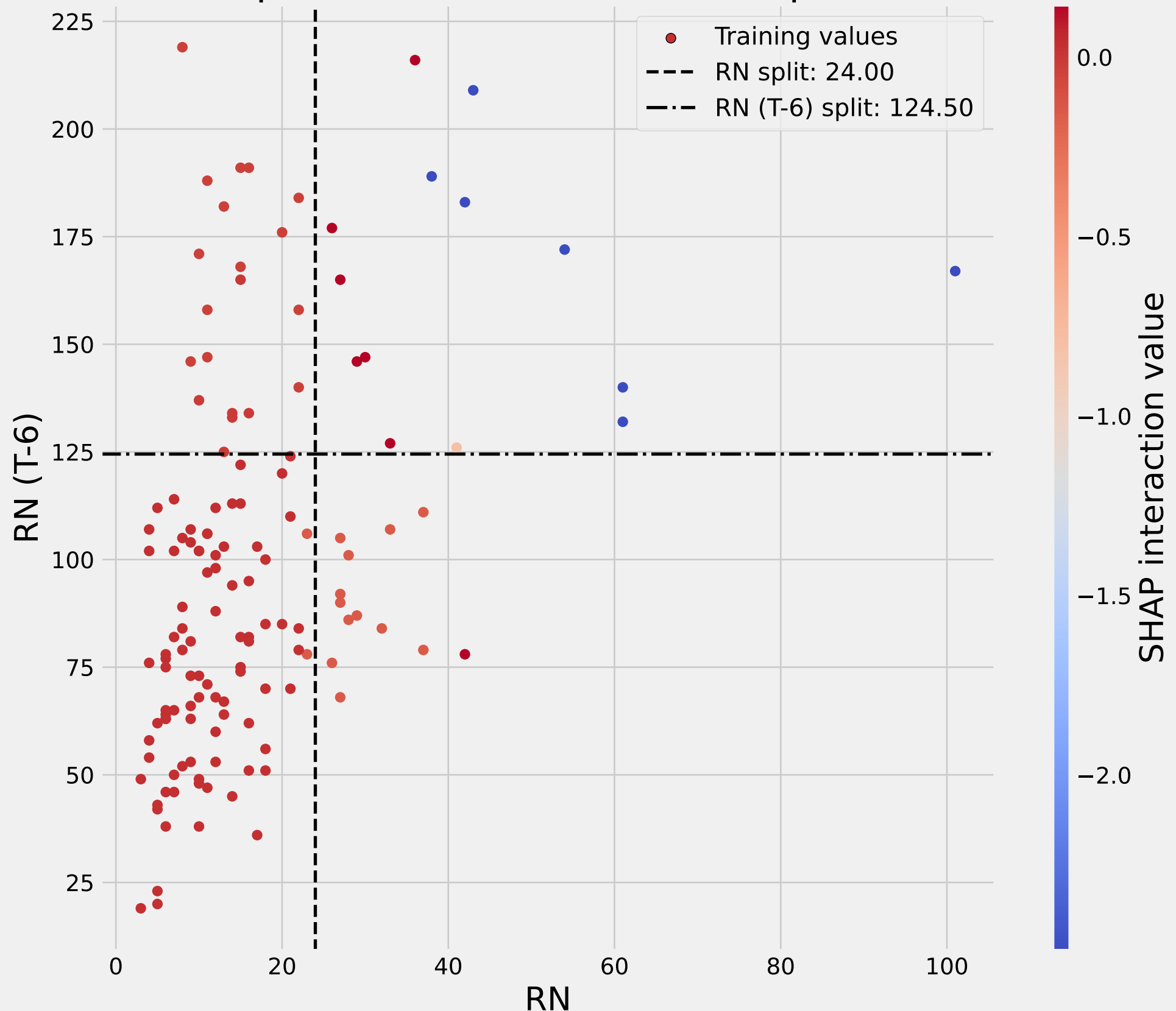
Optimal feature interaction splits
