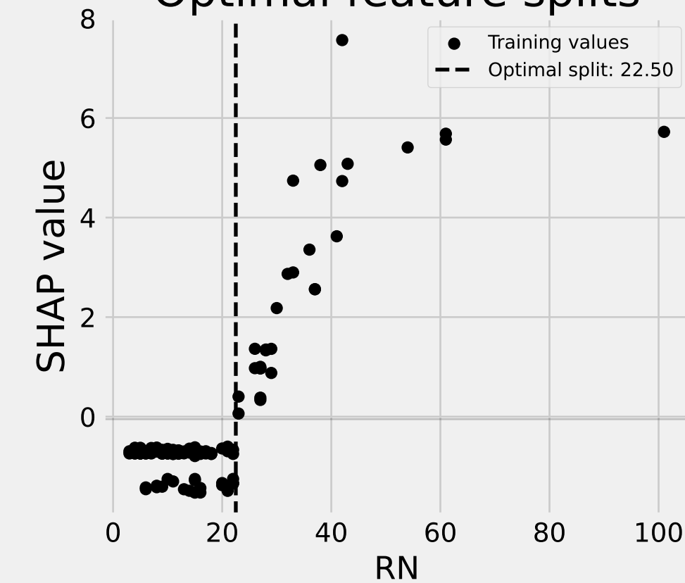
Optimal feature splits
