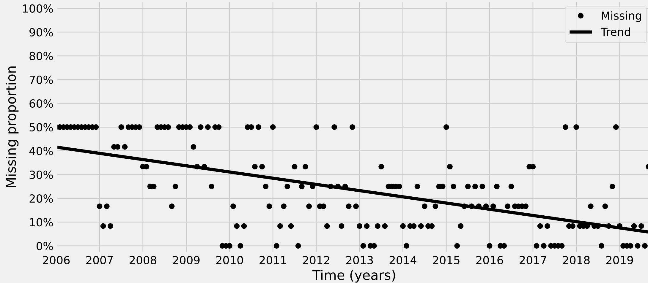
Proportion of missing bat-level observations
