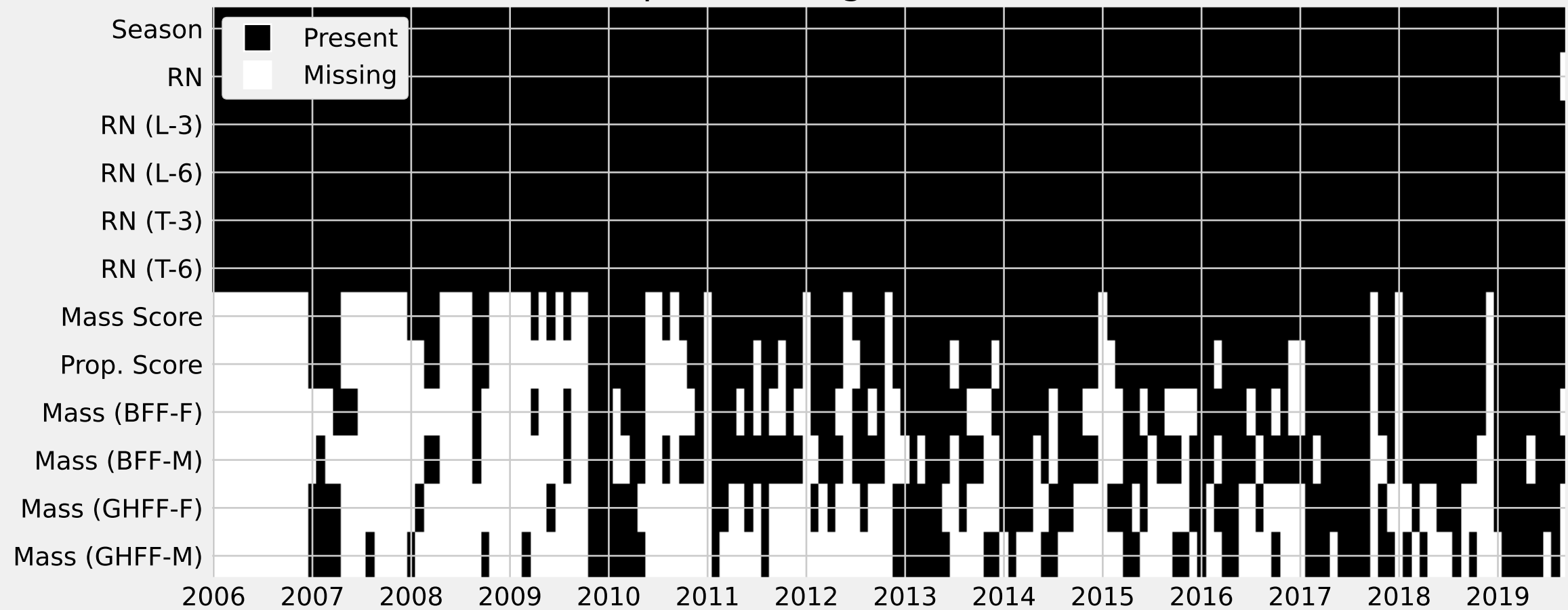
Heatmap of missing bat-level observations
