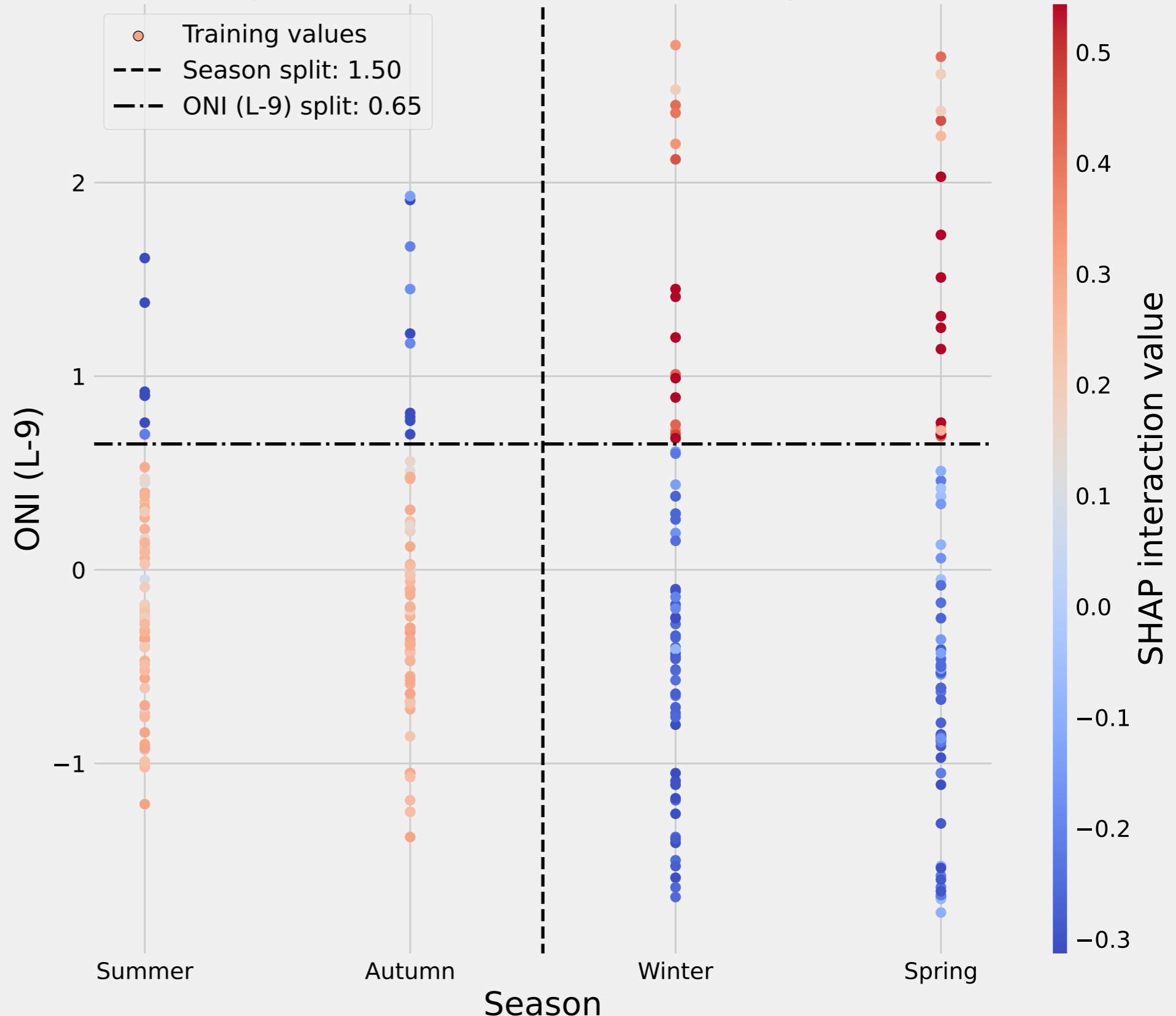
Optimal feature interaction splits
