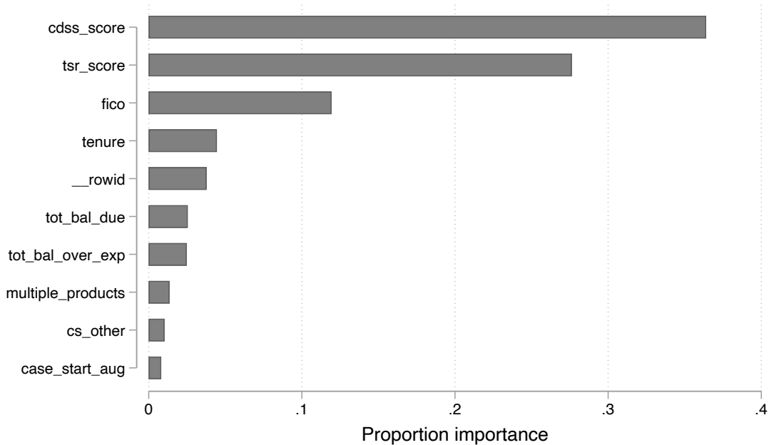
Variable importance plot using H2O
