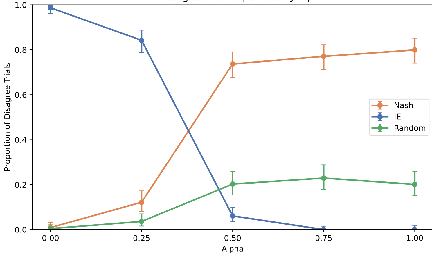
LLM Disagree-Trial Proportions by Alpha
