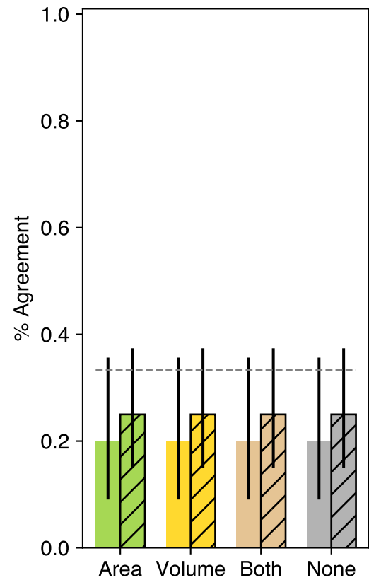
davinci-002
