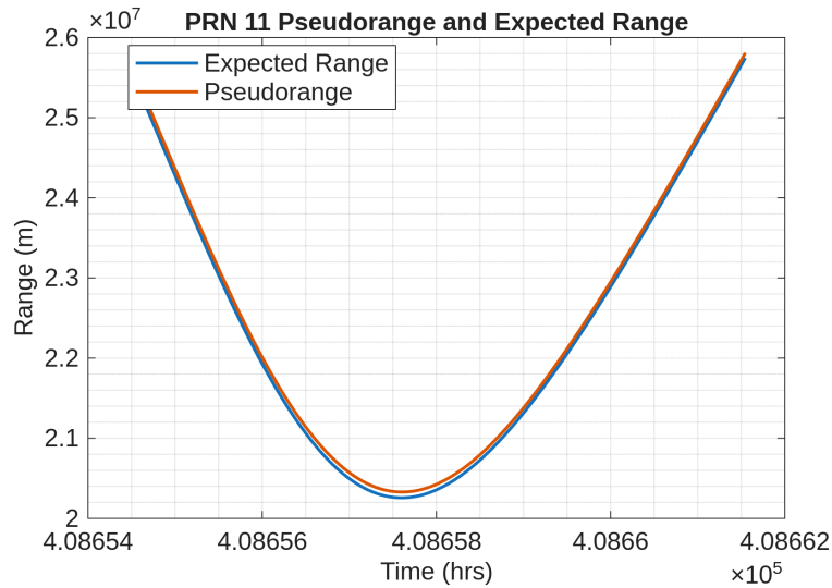
Figure 16: PRN11 C1C Pseudorange vs Expected Range
