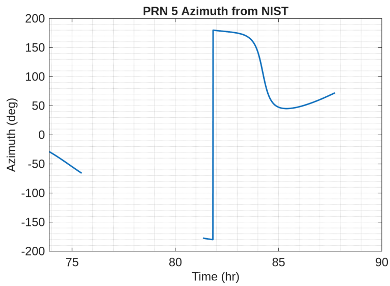
Figure 10: PRN5 Azimuth
