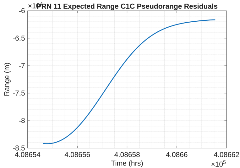
Figure 17: PRN11 C1C Pseudorange vs Expected Range Residuals
