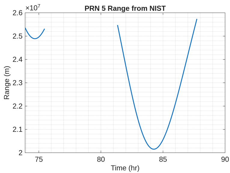
Figure 11: PRN5 Range
