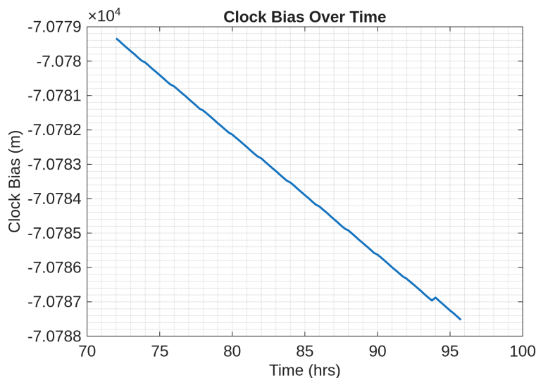
Figure 7: Clock Bias
