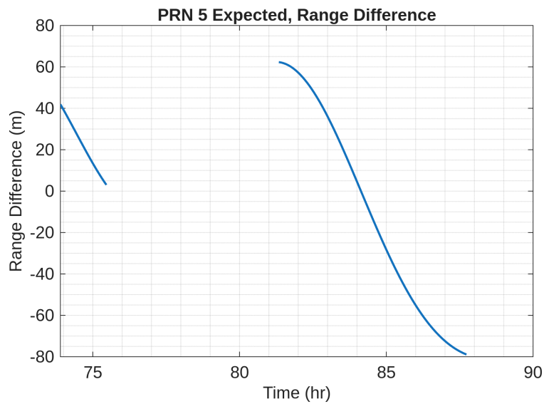
Figure 13: PRN5 Range Initial vs Expected Residual
