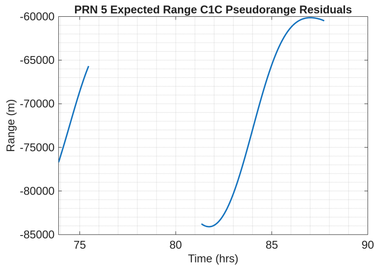
Figure 15: PRN5 C1C Pseudorange vs Expected Range Residuals
