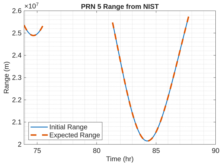
Figure 12: PRN5 Range Initial vs Expected
