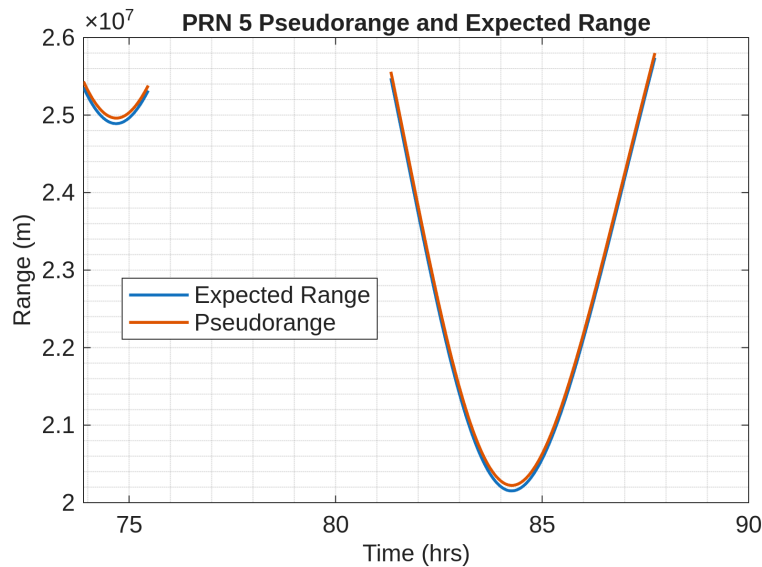
Figure 14: PRN5 C1C Pseudorange vs Expected Range
