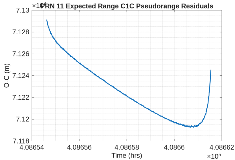
Figure 16: PRN11 C1C Pseudorange vs Expected Range Residuals
