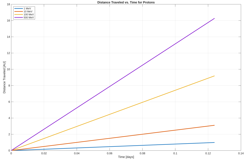
Figure 1: AU traveled vs time
