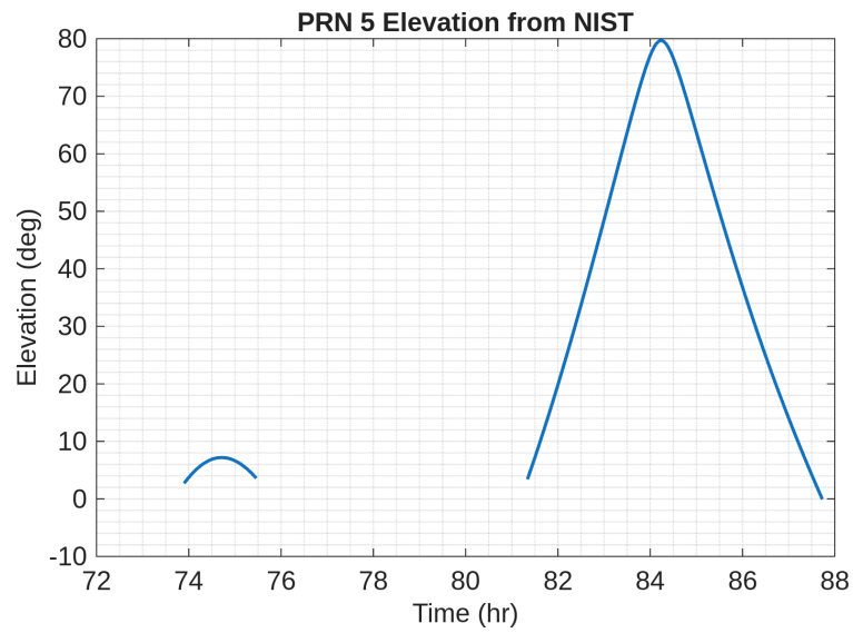
Figure 8: PRN5 Elevation
