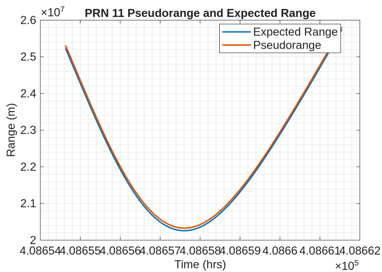
Figure 15: PRN11 C1C Pseudorange vs Expected Range
