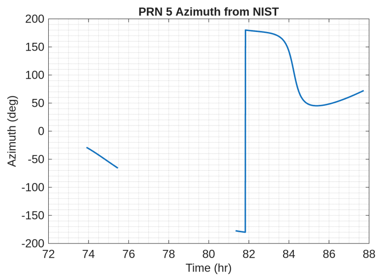
Figure 9: PRN5 Azimuth
