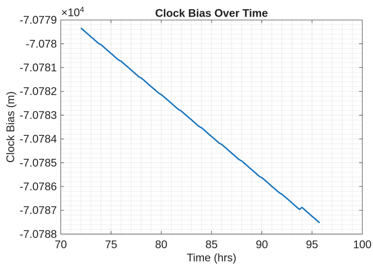
Figure 6: Clock Bias
