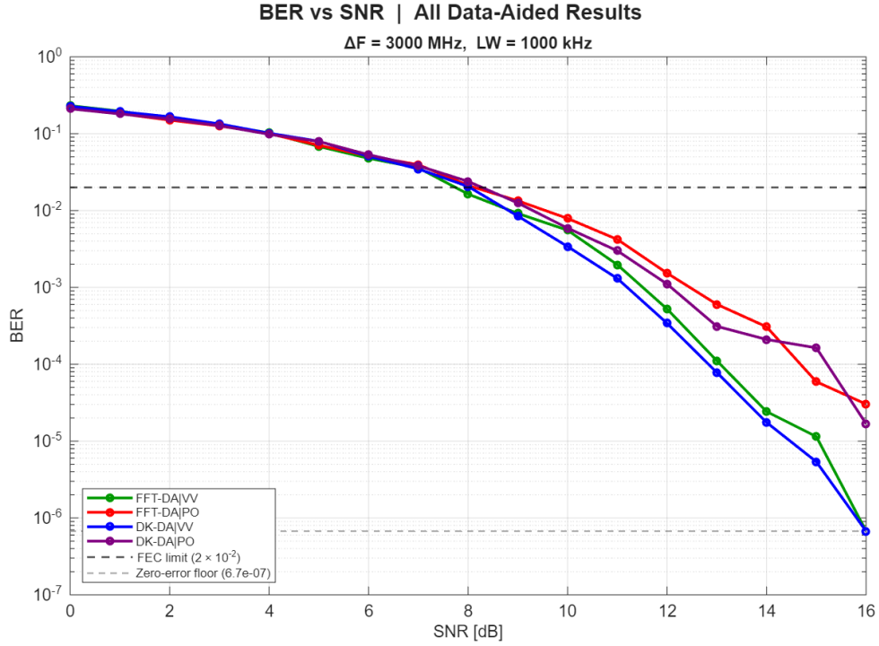
Figure 6: BER of carrier recovery combinations with f_d = 3 GHz and laser linewidth \Delta\nu = 1 MHz, R_s = 30.5 GBd, N_{FFT} = 512 .
