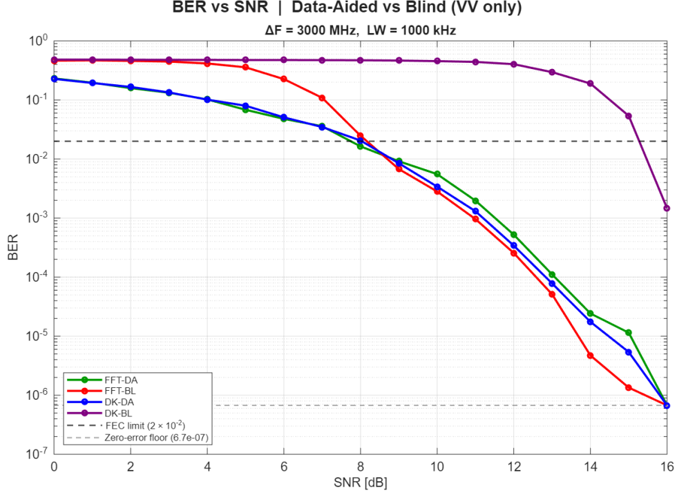
Figure 5: BER of data-aided vs blind frequency recovery with Viterbi & Viterbi.
