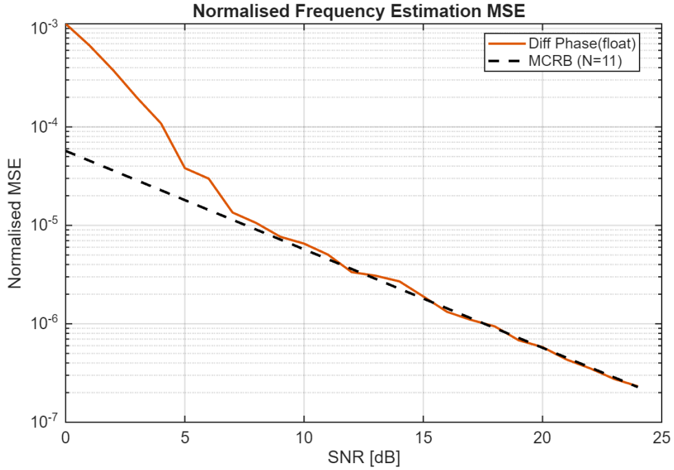
Figure 4: Normalised MSE of frequency estimation with the DK estimator for L = 11 training symbols.
