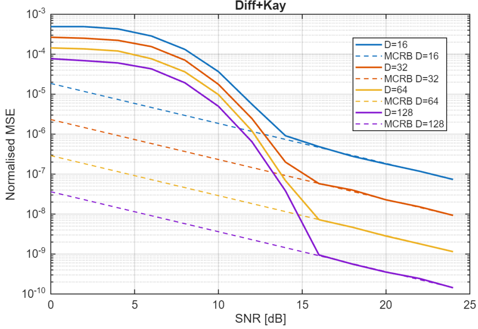
Figure 5: Normalised MSE of the DK estimator with blind operation for different observation lengths.
