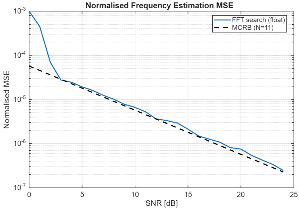
Figure 1: Normalised MSE of the R&B algorithm with FFT size N_{FFT} = 512 compared to the MCRB for L = 11 training symbols.
