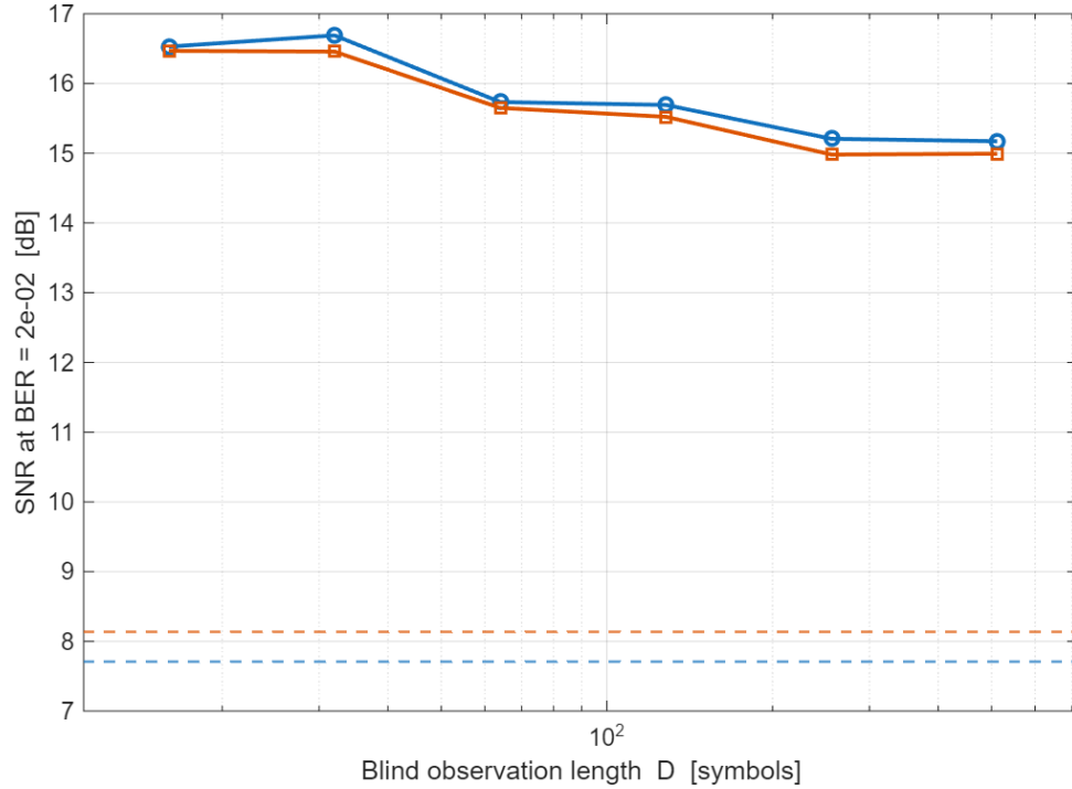
Figure 7: Threshold SNR vs blind observation length for the DK estimator. The dashed line is the threshold for data-aided operation. Orange: Pilots-Only. Blue: Viterbi & Viterbi.
