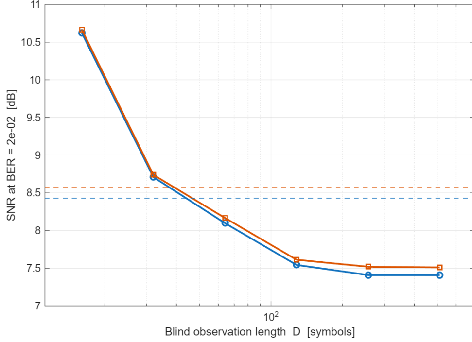
Figure 6: Threshold SNR vs blind observation length for the R&B algorithm. The dashed line is the threshold for data-aided operation. Orange: Pilots-Only. Blue: Viterbi & Viterbi.
