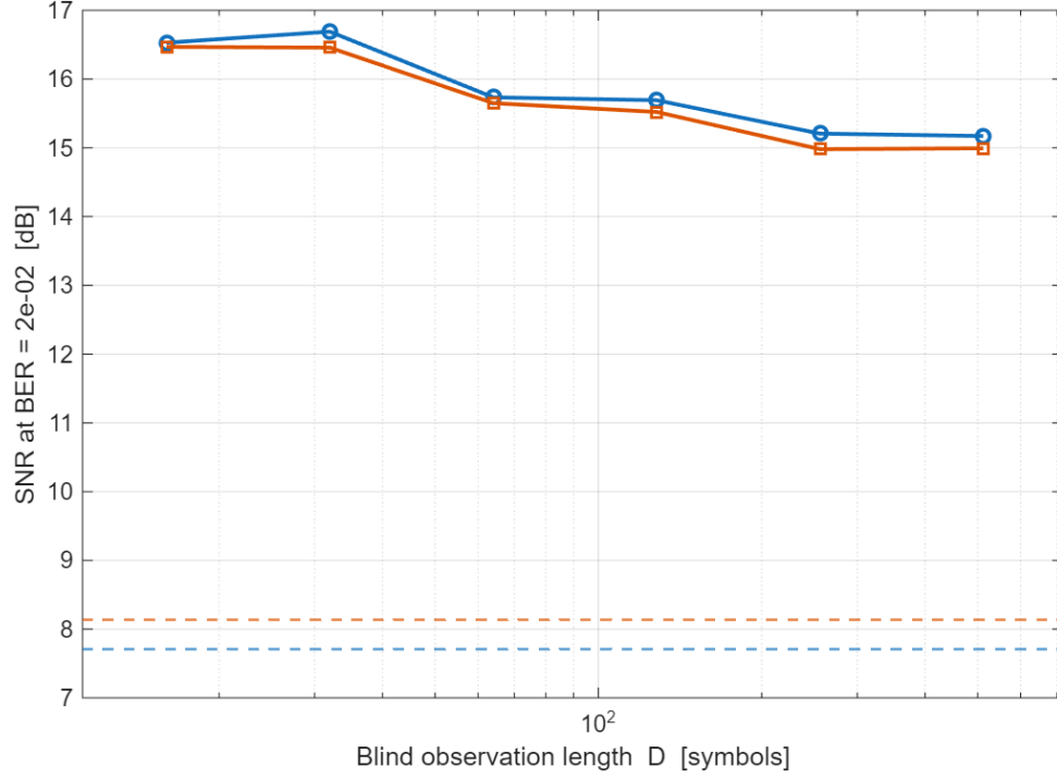
Figure 7: FEC SNR vs blind observation length for the DK estimator. The dashed line is the FEC SNR for data-aided operation. Orange: Pilots-Only. Blue: Viterbi & Viterbi.
