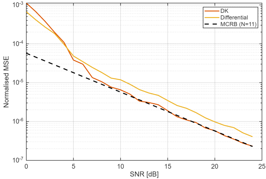
Figure 4.3: Normalised MSE of frequency estimation with the DK estimator for L = 11 training symbols.
