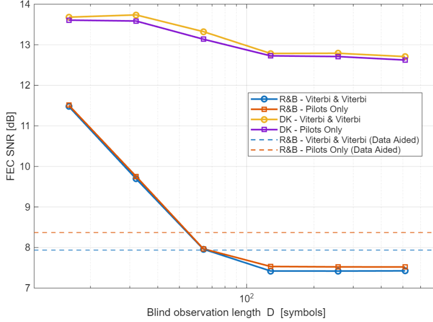
Figure 4.7: FEC SNR vs blind observation length for the R&B and DK estimators. CFO = 2 GHz, laser linewidth = 1 MHz.
