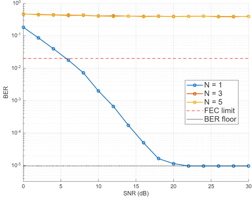
Figure 3.1: BER vs SNR for adaptive equaliser tap lengths of 1,3,5 using CMA and direct update at 16 bits of precision.
