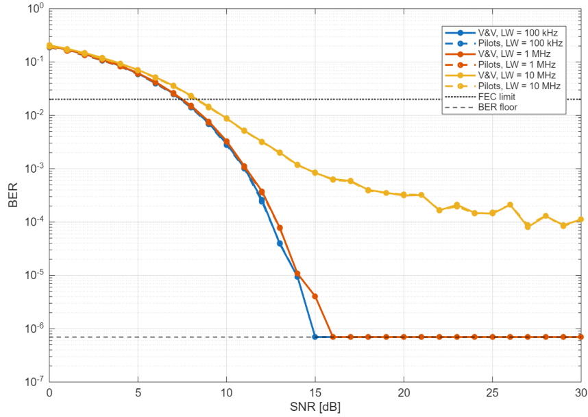
Figure 2.6: Performance comparison of V&V and Pilots-Only phase correction
