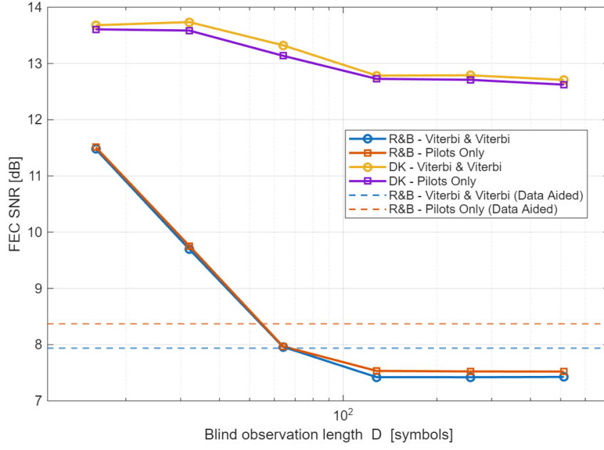
Figure 2.7: FEC SNR vs blind observation length for the R&B and DK estimators. CFO = 2 GHz, laser linewidth = 1 MHz
