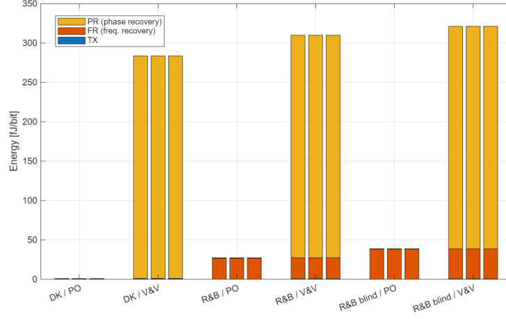
(a) Shot-noise limited (10 km passive-split PON).
