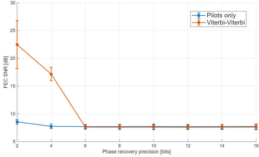
(a) FEC SNR
