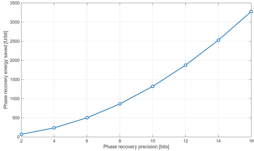
(b) Energy saved by switching V&V \rightarrow pilots-only
