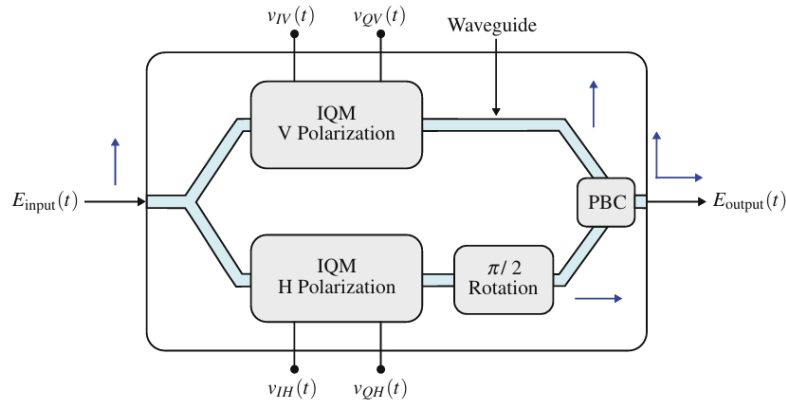
Figure 2.2: Dual-polarisation coherent modulator using MZMs.
