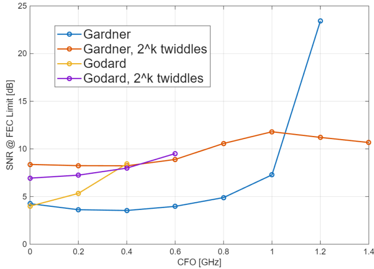
Figure 3.1: SNR @ FEC limit as CFO varies for each implementation. Points are omitted when the FEC limit is no longer reached at any SNR.
