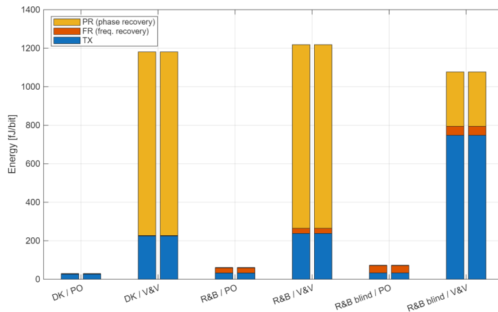
Figure 3.8: Energy breakdown for carrier recovery. Left: (20 km, 1:512). Right: (80 km, 1:16).
