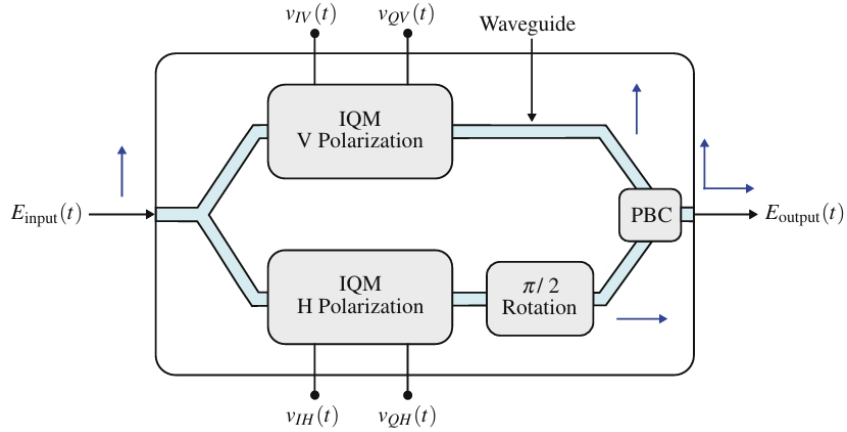
Figure 5.1: Dual-polarisation coherent modulator using MZMs.
