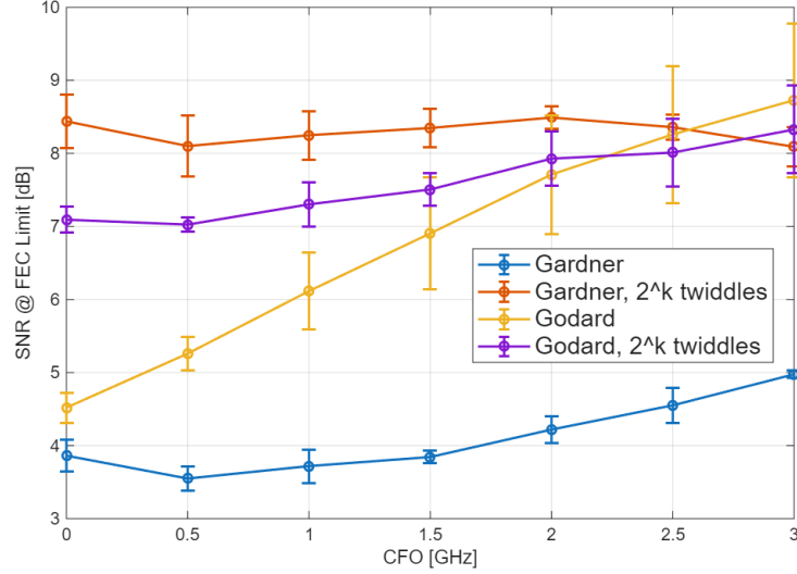
Figure 3.2: SNR @ FEC limit as CFO varies with coarse CFO correction.
