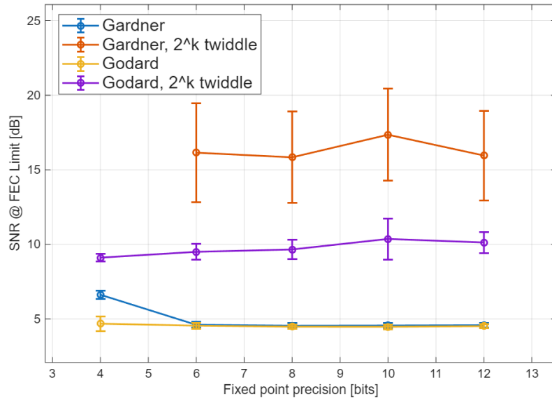
Figure 3.5: RSNR as the fixed-point precision of clock recovery varies, with static and adaptive equalisation at high precision.
