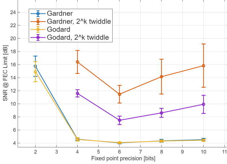
Figure 3.3: RSNR as the fixed-point precision of adaptive equalisation varies, with static equalisation and clock recovery at high precision.
