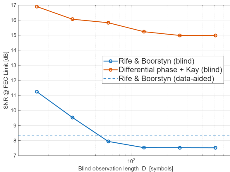
Figure 4.8: RSNR vs blind observation length for the Rife & Boorstyn and differential phase and Kay estimators.
