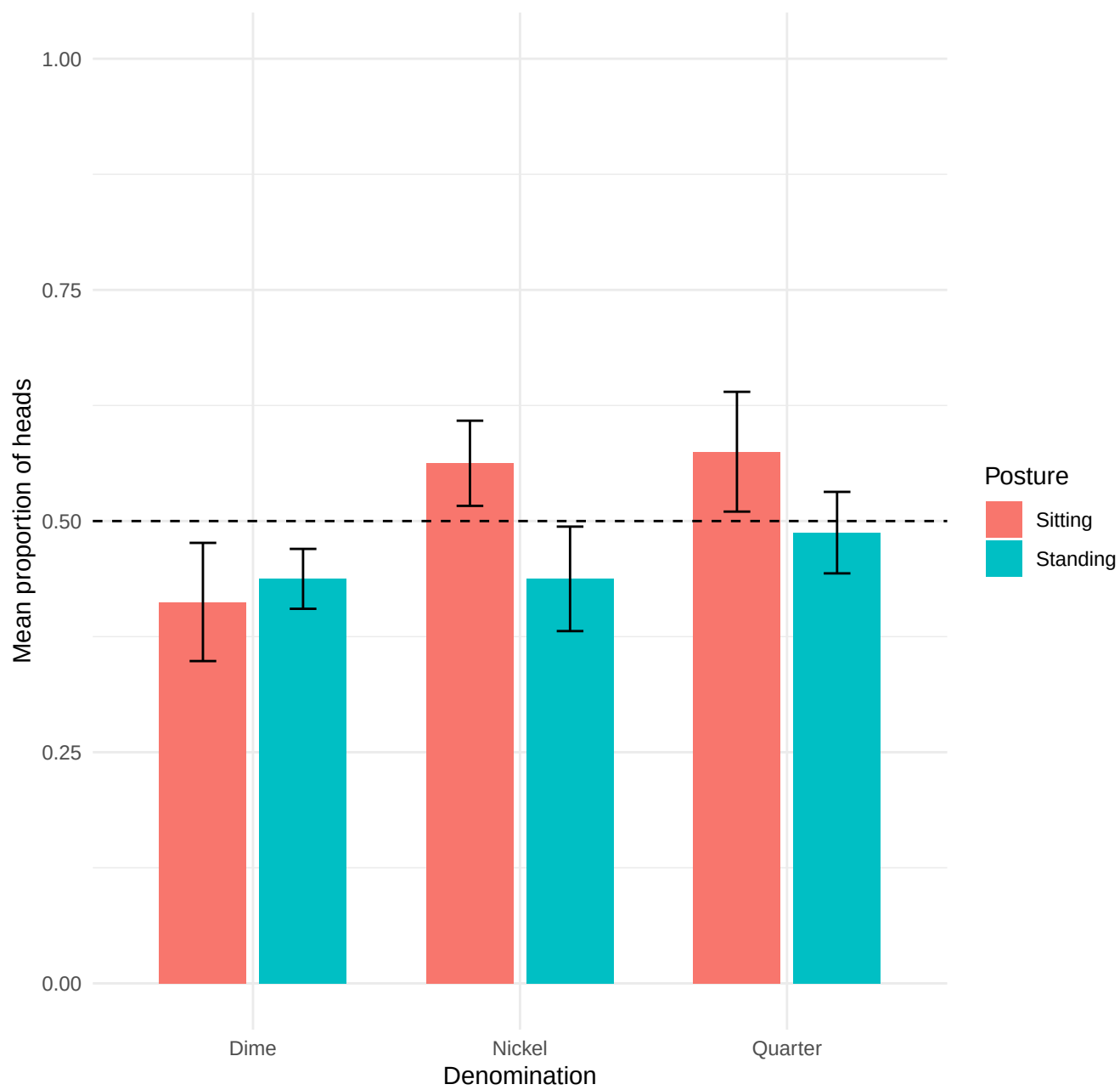
Mean proportion of heads by treatment
